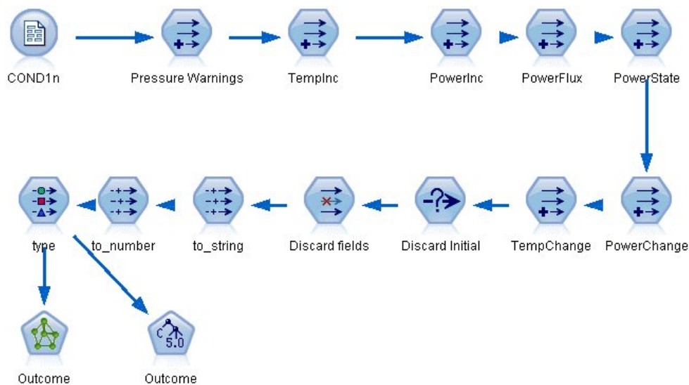
Figure 262. Condlearn stream
