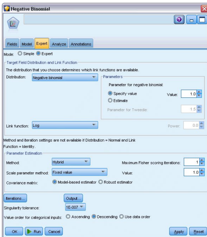
Figure 319. Expert tab
