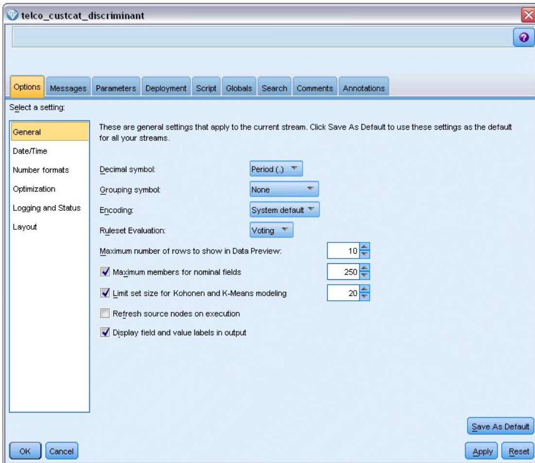
Figure 265. Stream properties
