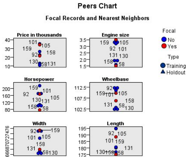
Figure 393. Peers chart
