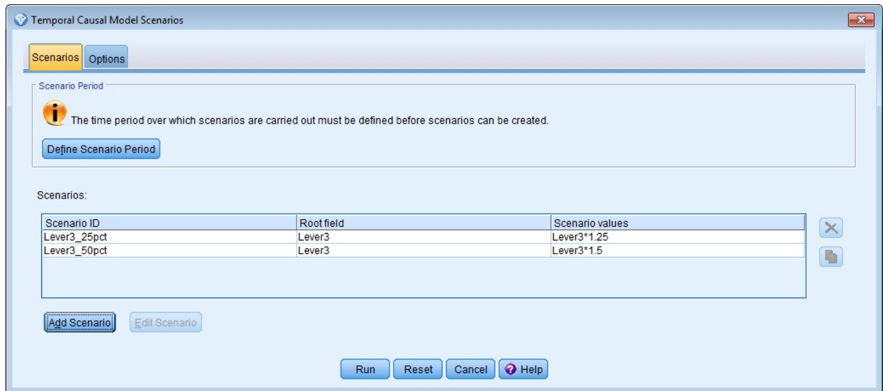
Figure 411. Scenarios
