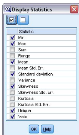
Figure 66. Display Statistics
