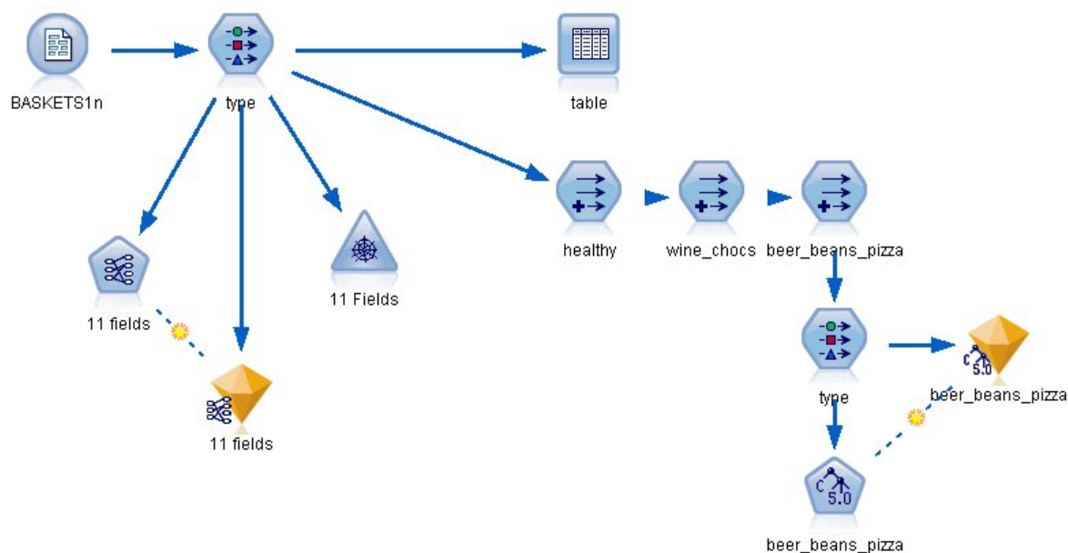
Figure 380. baskrule stream
