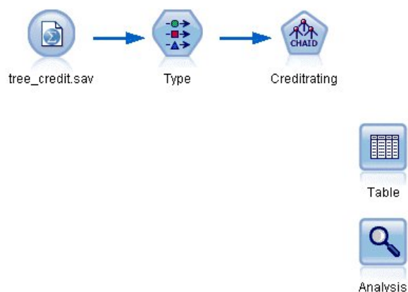
Figure 12. Modeling stream
